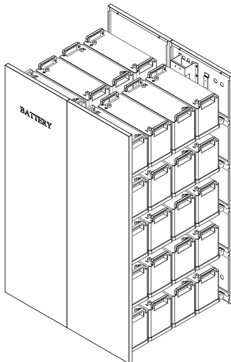
40pcs Batteries 100AH/120AH 407 × 176 × 136(L × W × H)
